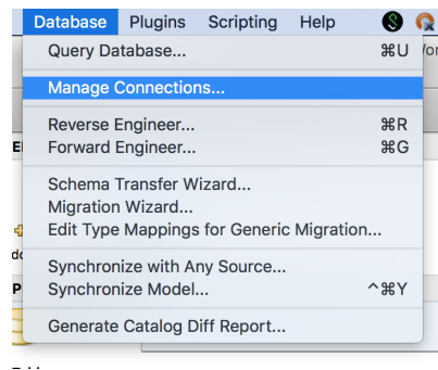
FIGURA 2.3. Manage connections
